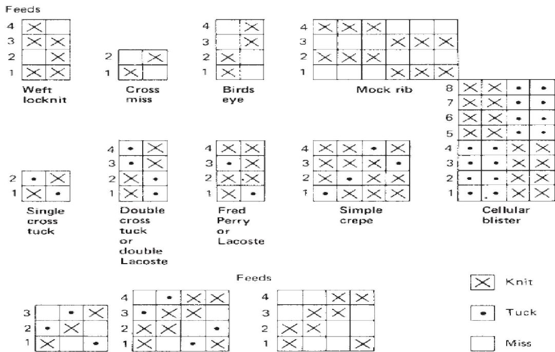
Fig. 13.1 Twill effects.
